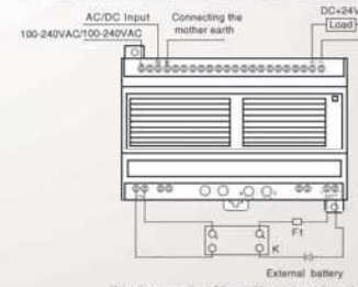
(Attn: the connection of the positive and negative pole) (Fig.3.4: Using Remote and UPS simultaneously application)
